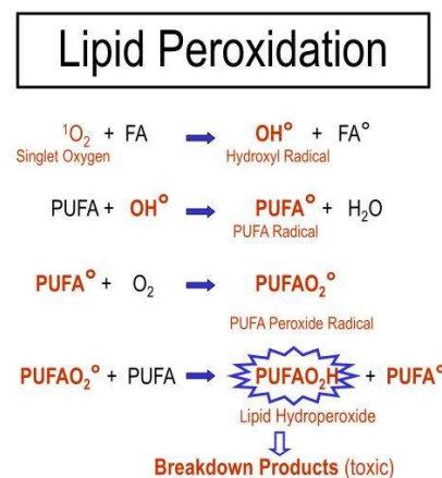
Figure 1. The lipid peroxidation. FA = fatty acid, PUFA = polyunsaturated fatty acids.
